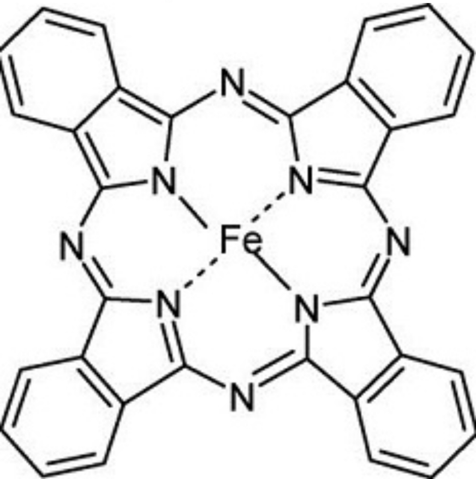
Ferrous Phthalocyanine (FePc)
